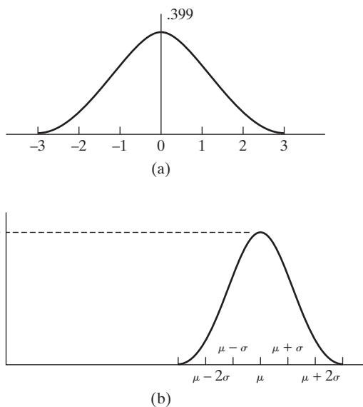
Figure 5.5 Normal density function: (a) \mu = 0, \sigma = 1 ; (b) arbitrary \mu, \sigma^2 .
